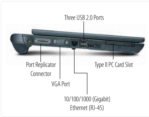
LEFT VIEW
